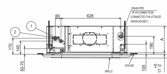
PLA-SM71/100/125/140
